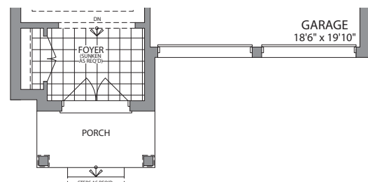
MAIN FLOOR ELEVATION C
