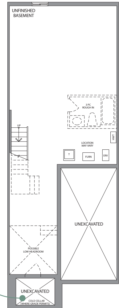
BASEMENT ELEVATION A & B
